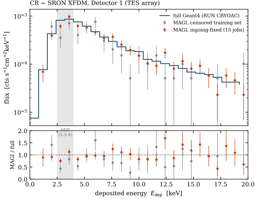
Figure 3: CR at detector level, SRON XFDM Detector 1. Full Geant4 (RUN CRYOAC) against MAGI trained on the censored (3 jobs) and on the ingoing-fixed set (15 jobs, pooled from cr_retest and cr_retest_morestat ), in flux units with the Fig. 1(b) normalisation. Each MAGI crossing stands for 1/\chi primaries, and \chi differs between the two checkpoints — which is the effect under test. Shaded band: MIP, 2.5–4 keV.
