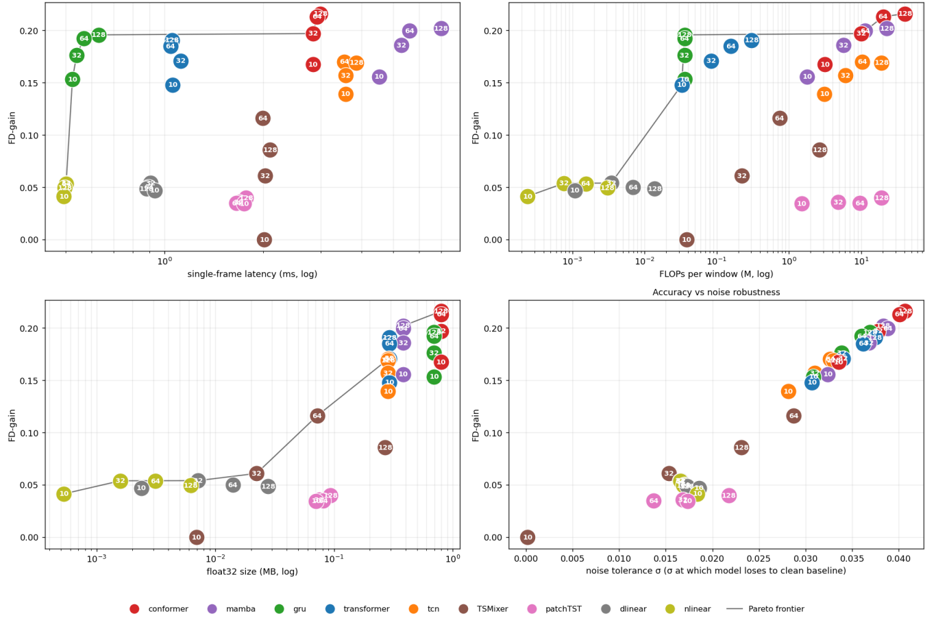
FIG. 7: Pareto-optimal frontier visualizations. FD_{gain} (accuracy) is plotted against the different cost axes (latency, FLOPs, size) and against noise tolerance. The conformer leads on accuracy, the mamba follows, and the GRU offers the best accuracy-per-latency trade-off.
