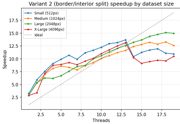
Figure 3: Speedup of Variant 2 (border/interior split) across the four dataset sizes.
