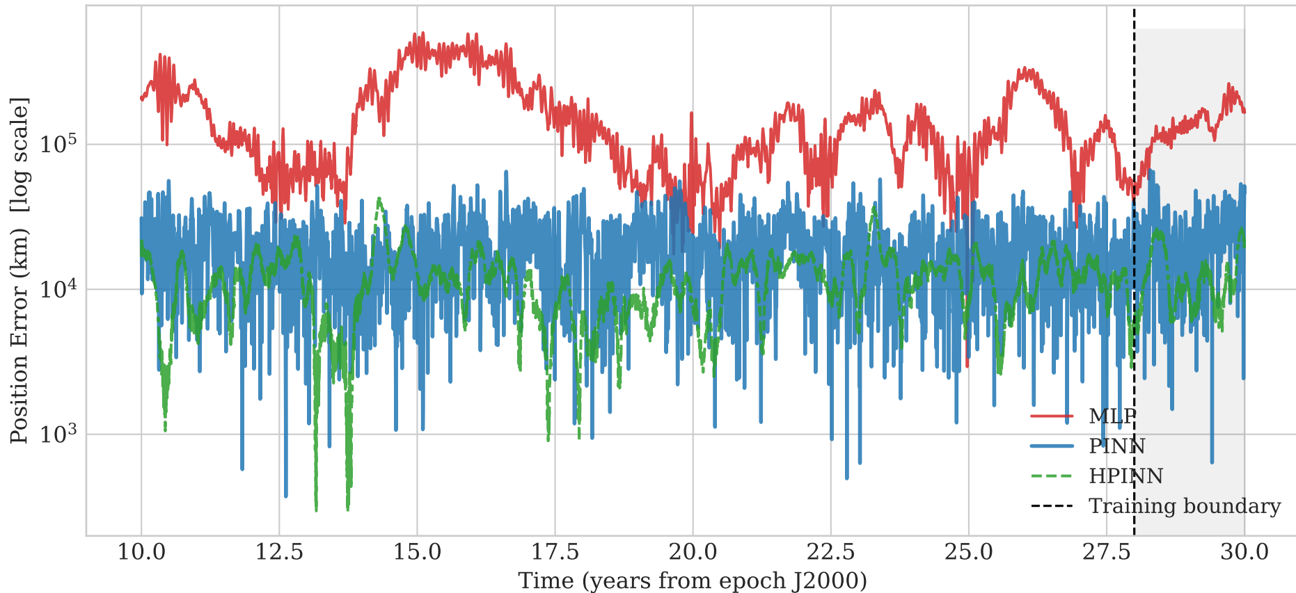
Long-Term Extrapolation Error — Earth (body #3)
