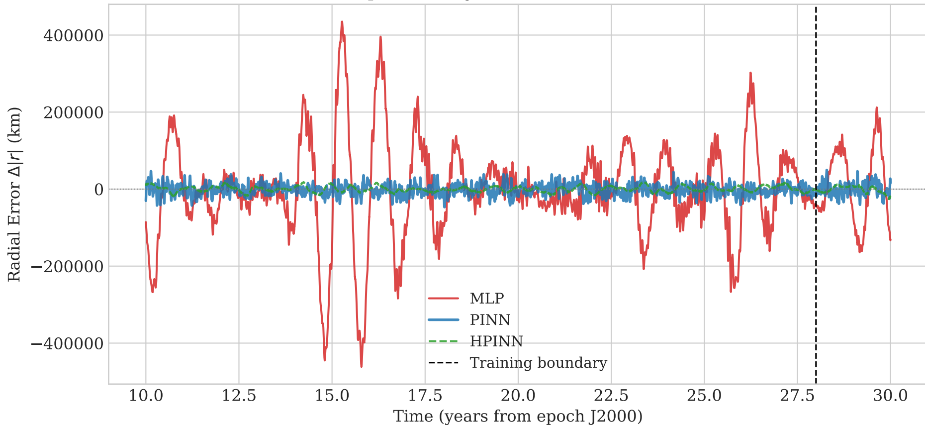
Orbital Shape Stability: Radial Distance Error — Earth
