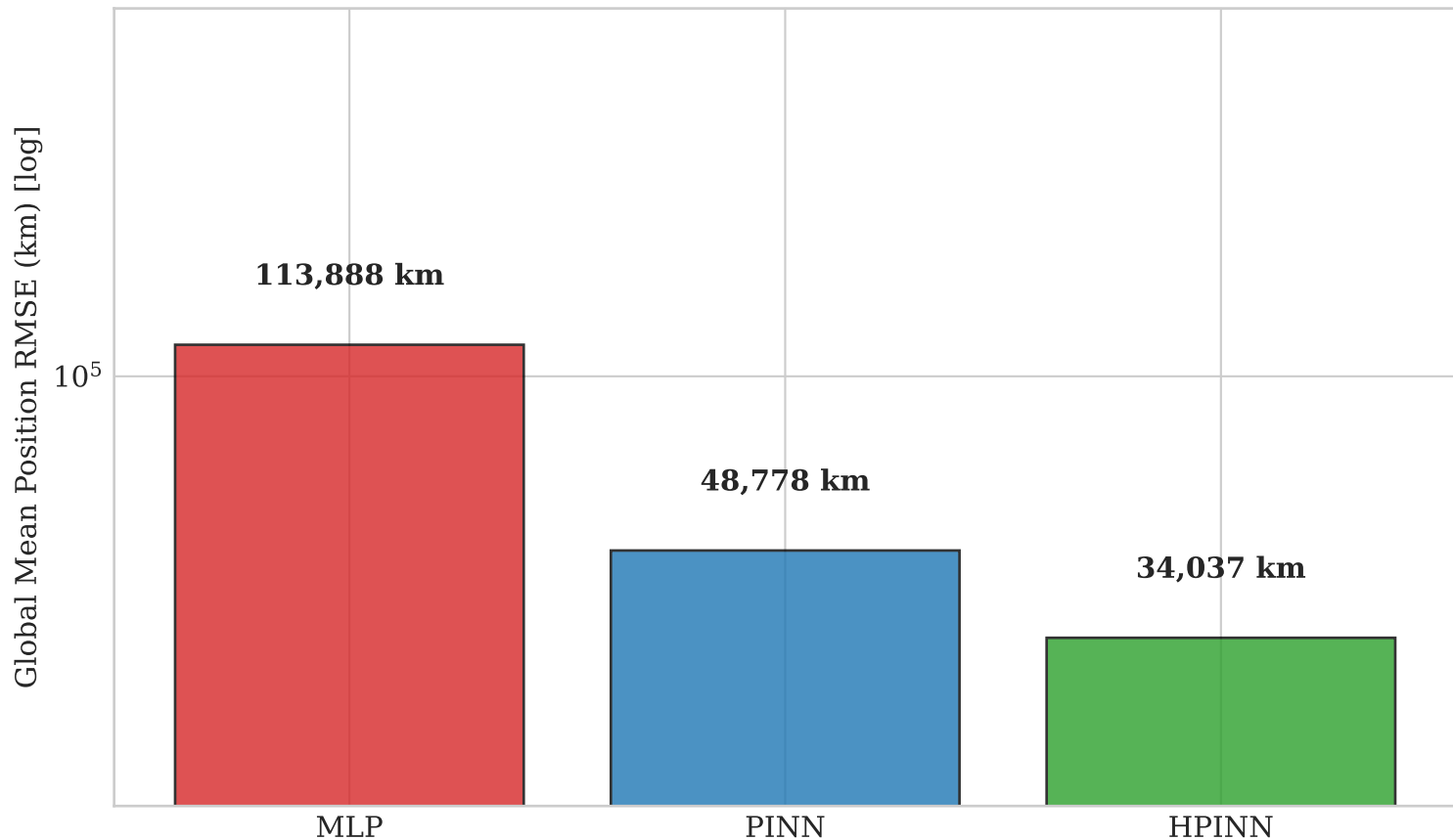
Global Benchmark: MLP vs PINN vs HPINN
