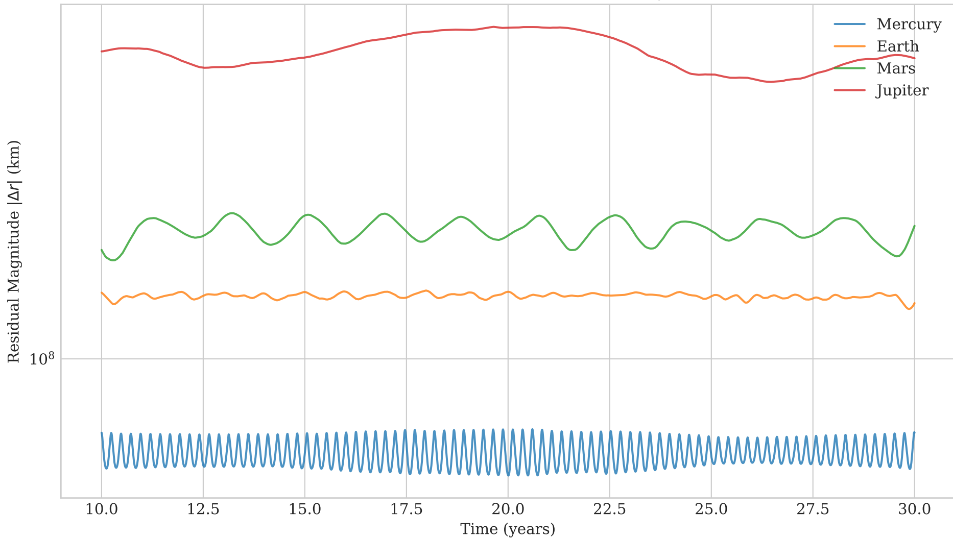
Learned Corrections to Newtonian Physics
