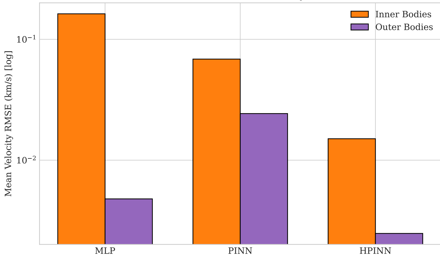
Inner vs Outer Bodies: Velocity Error
