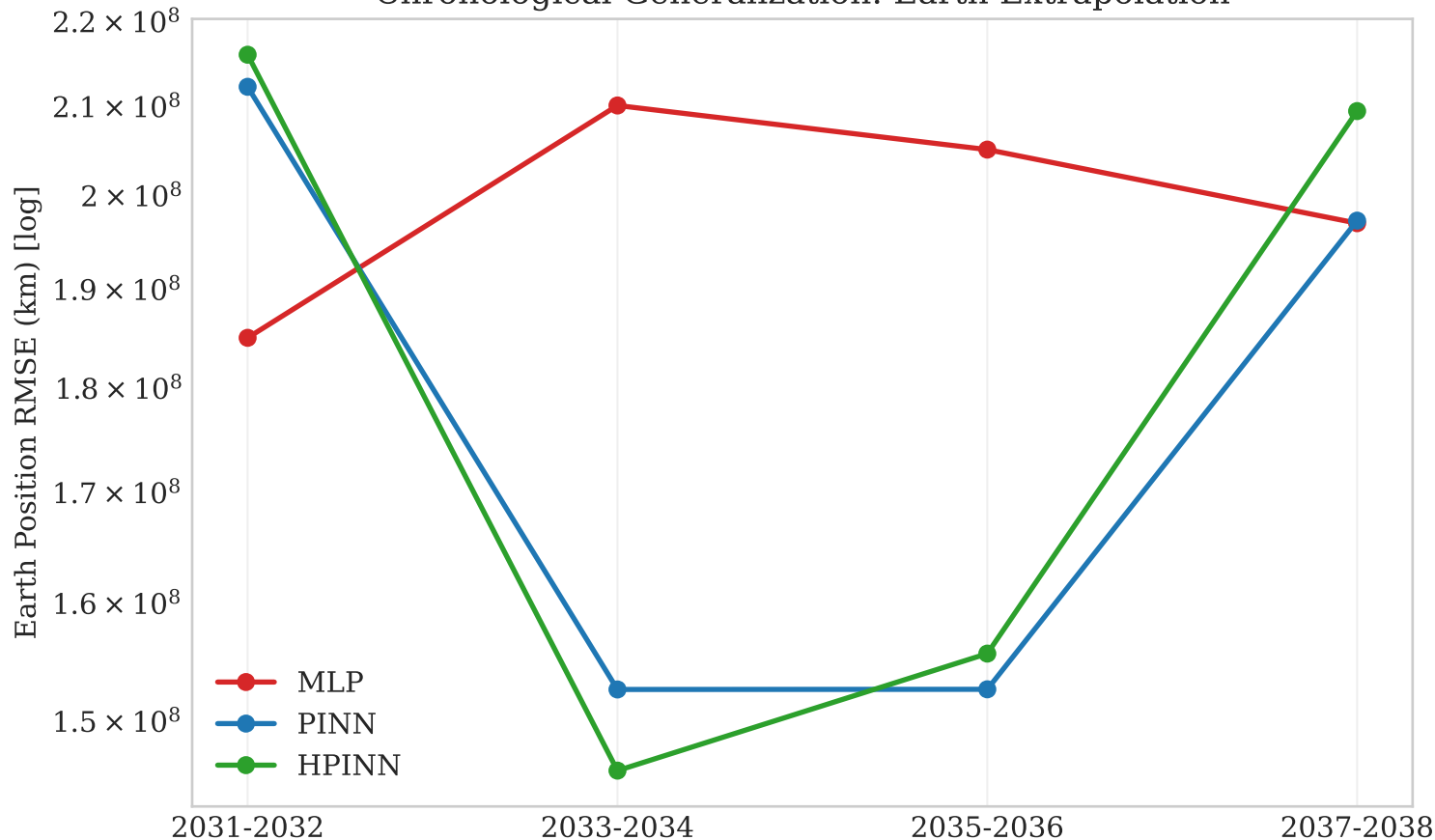
Chronological Generalization: Earth Extrapolation
