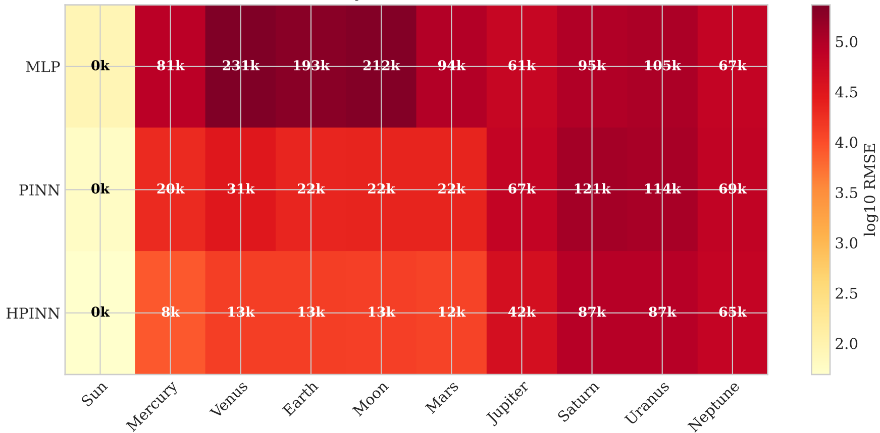
Per-Body Position RMSE (km)
