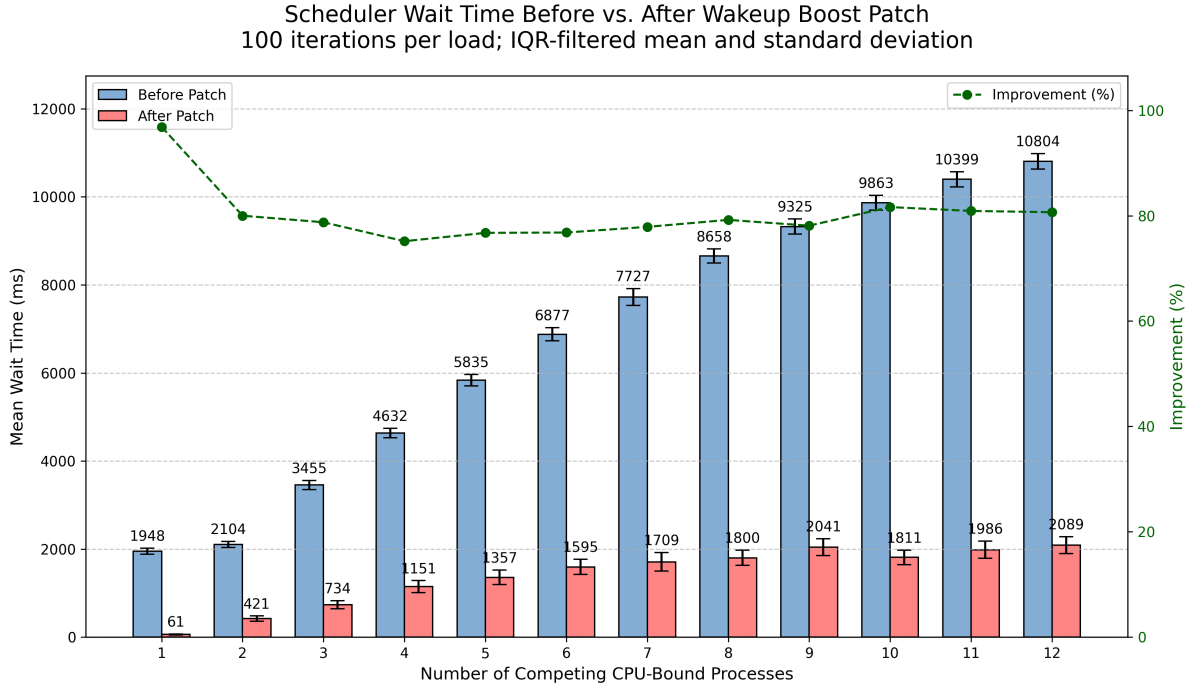
Figure 1: Target-task runnable wait time before and after the wakeup boost. Error bars show the standard deviation after per-scenario IQR filtering.
