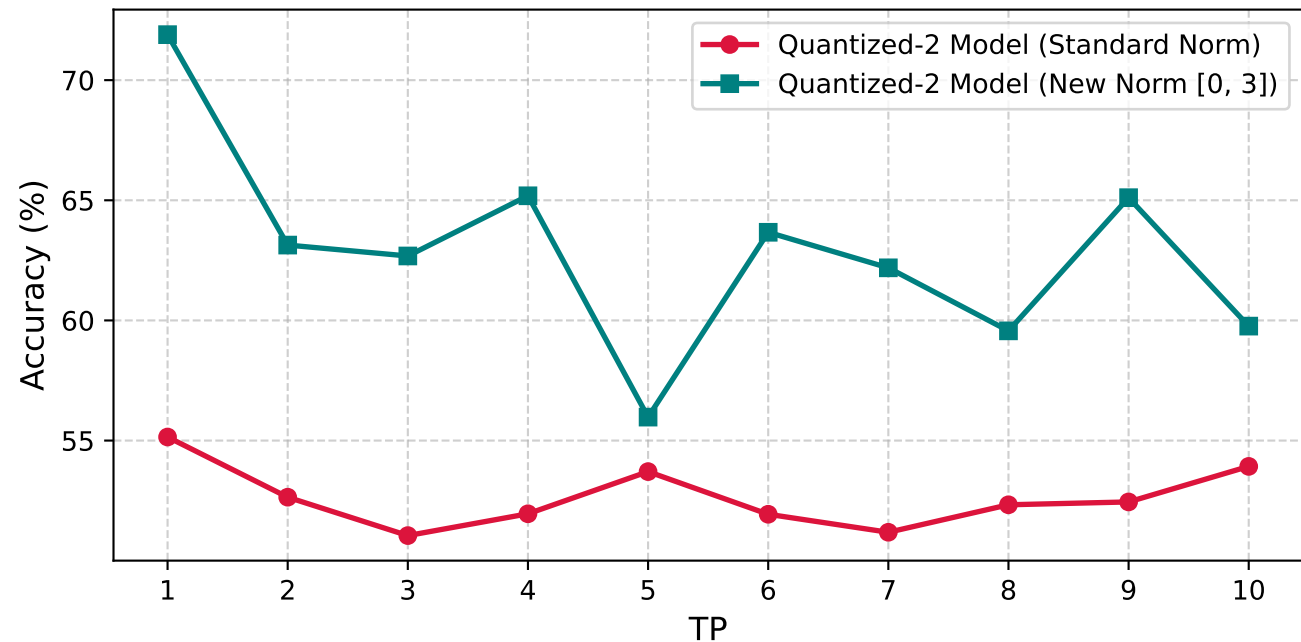
Test Accuracy Comparison: Quantized-2 Model vs New Norm Model)
