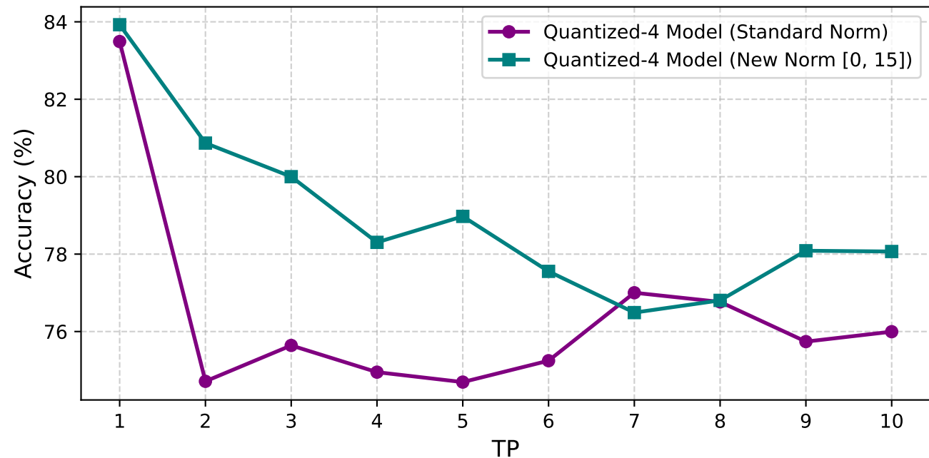
Test Accuracy Comparison: Quantized-4 Model vs New Norm Model)
