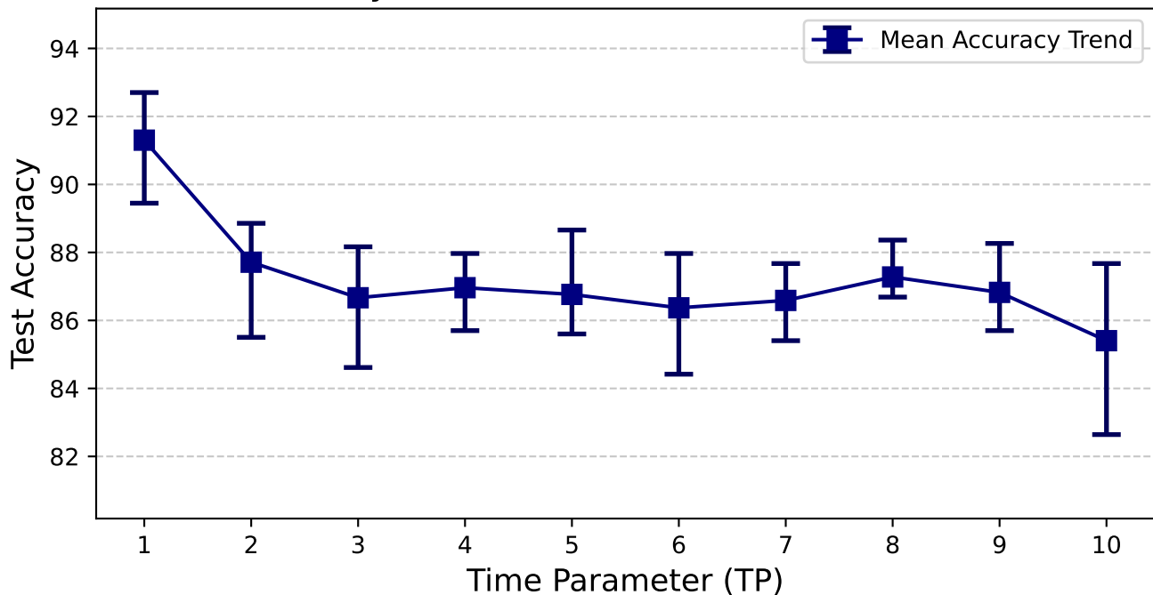
Test Accuracy Trend Baseline CNN vs TP - Scheduler 3
