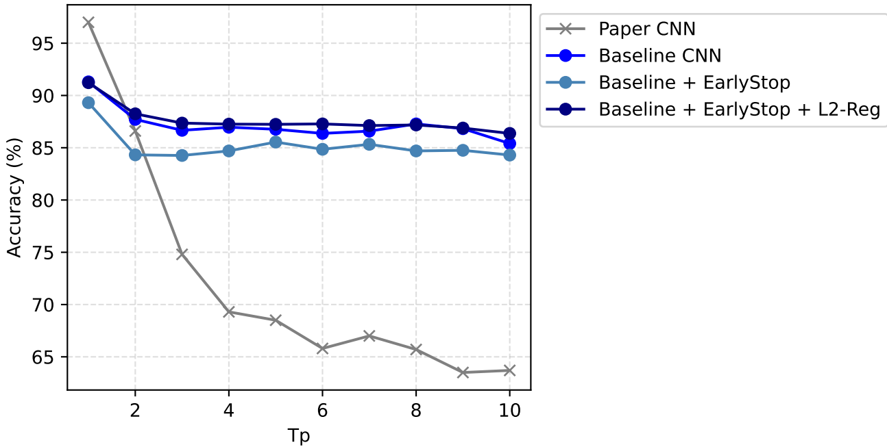
Test Accuracy vs Tp
