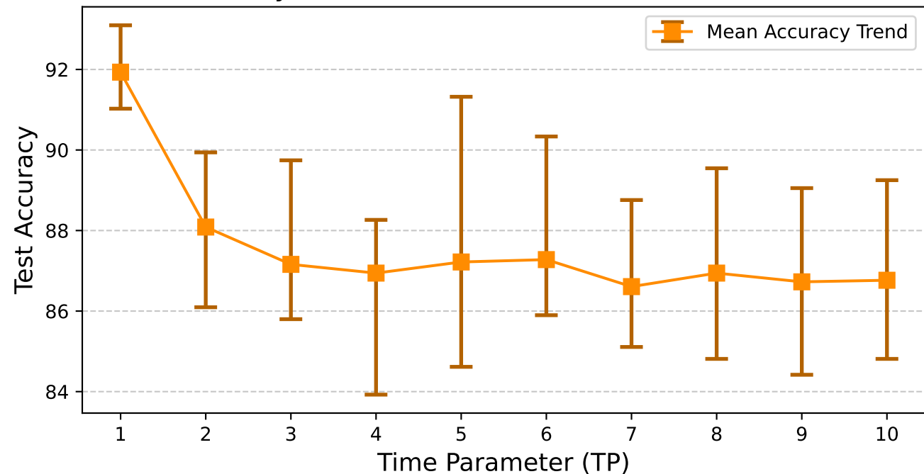
Test Accuracy Trend Constrained CNN vs TP - Scheduler 3
