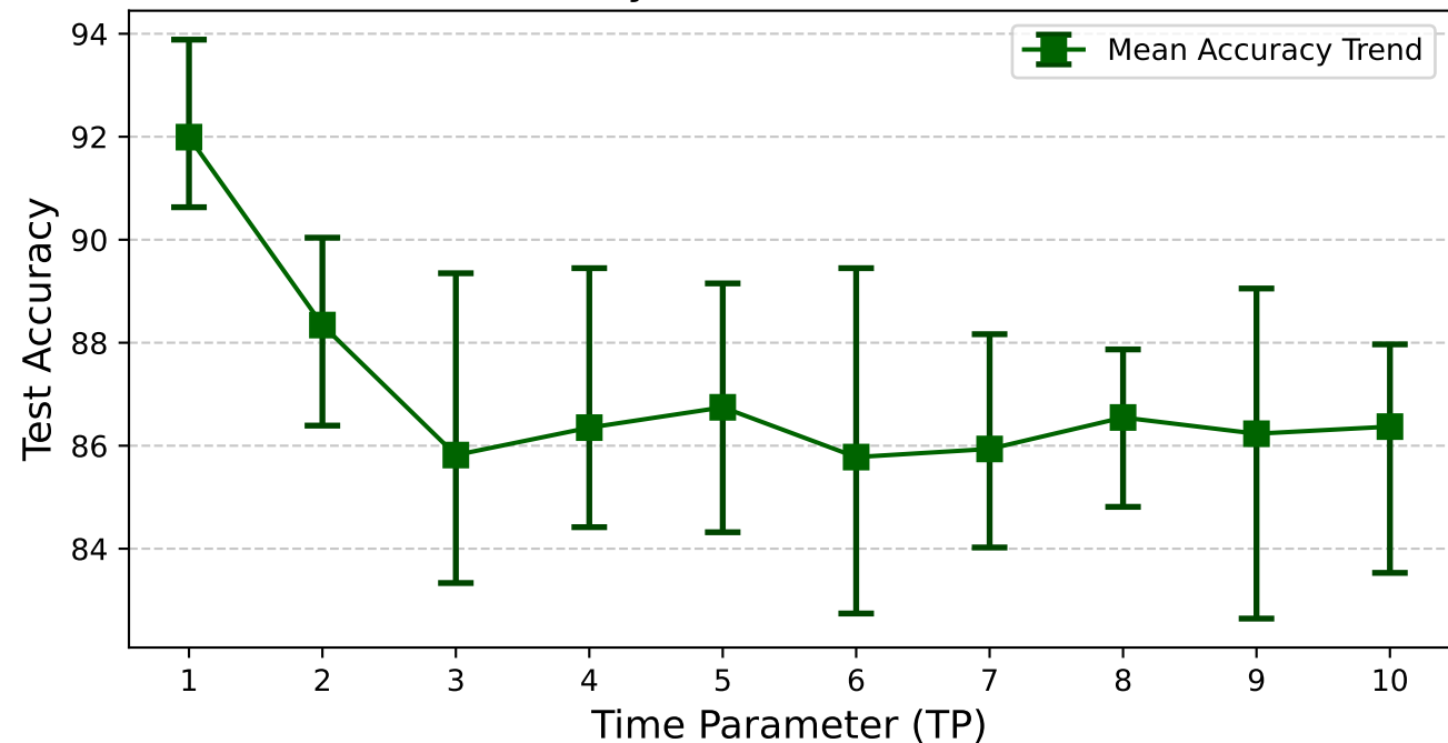
Test Accuracy Trend vs TP - Scheduler 3
