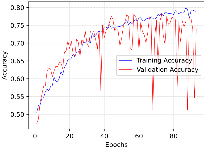
Training VS. Validation Accuracy Quantized-4-Large Model - Tp=10 - Seed=1
