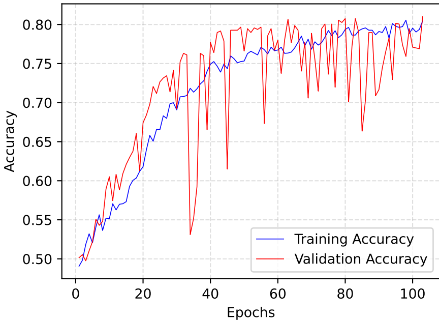
Training VS. Validation Accuracy Quantized-4-Large Model - Tp=2 - Seed=1
