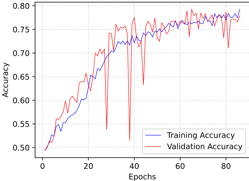
Training VS. Validation Accuracy Quantized-4-Large Model - Tp=3 - Seed=1
