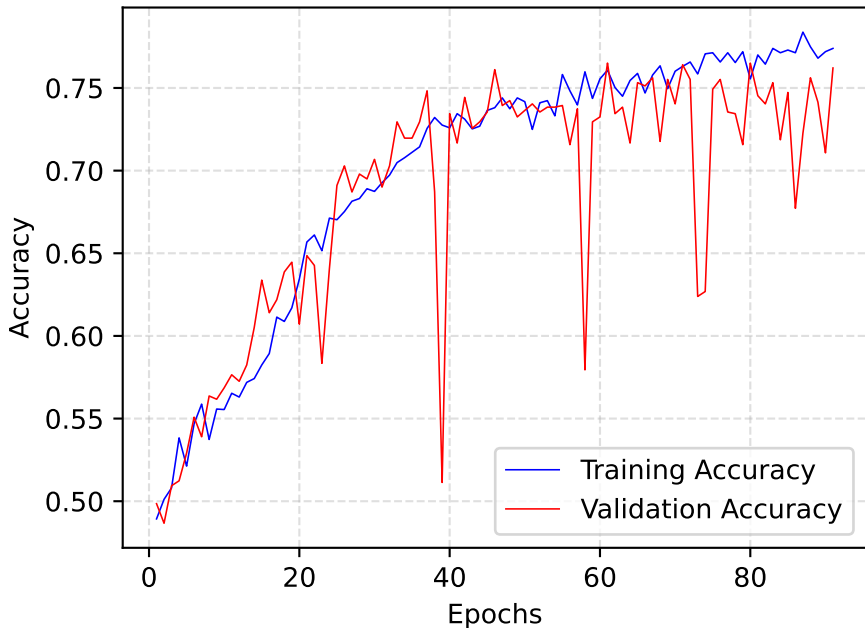
Training VS. Validation Accuracy Quantized-4-Large Model - Tp=5 - Seed=1
