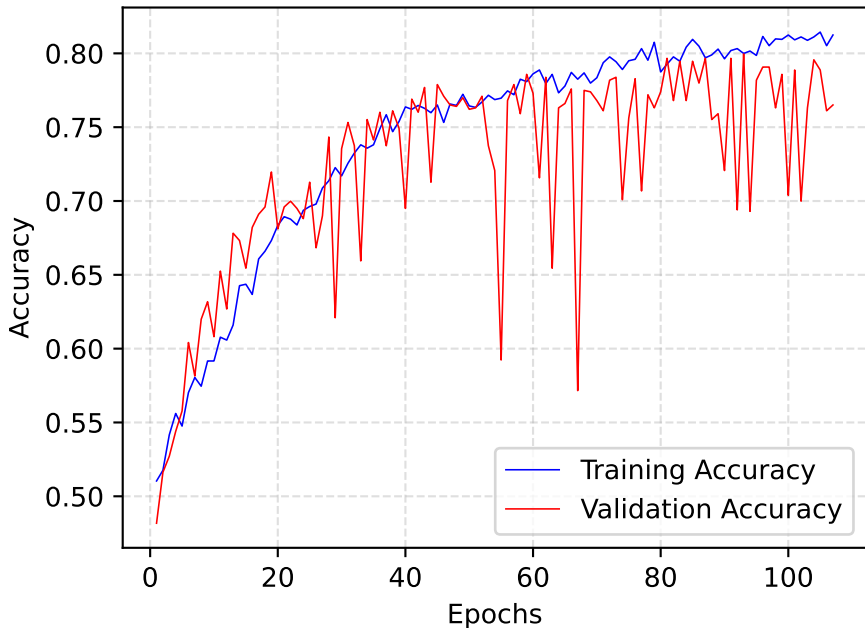
Training VS. Validation Accuracy Quantized-4-Large Model - Tp=7 - Seed=1
