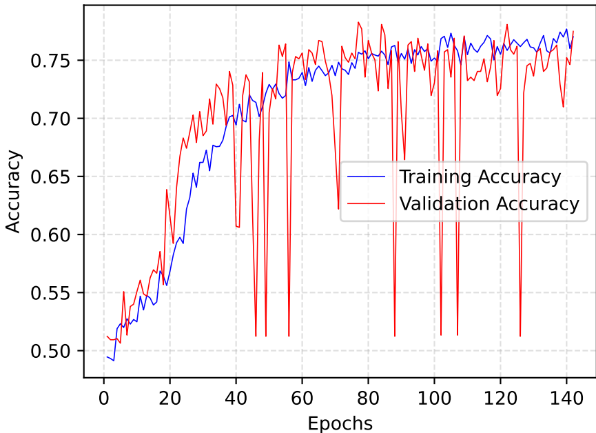
Training VS. Validation Accuracy Quantized-4-Small Model - Tp=10 - Seed=1
