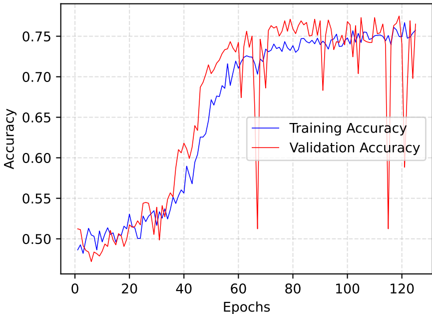
Training VS. Validation Accuracy Quantized-4-Small Model - Tp=3 - Seed=1
