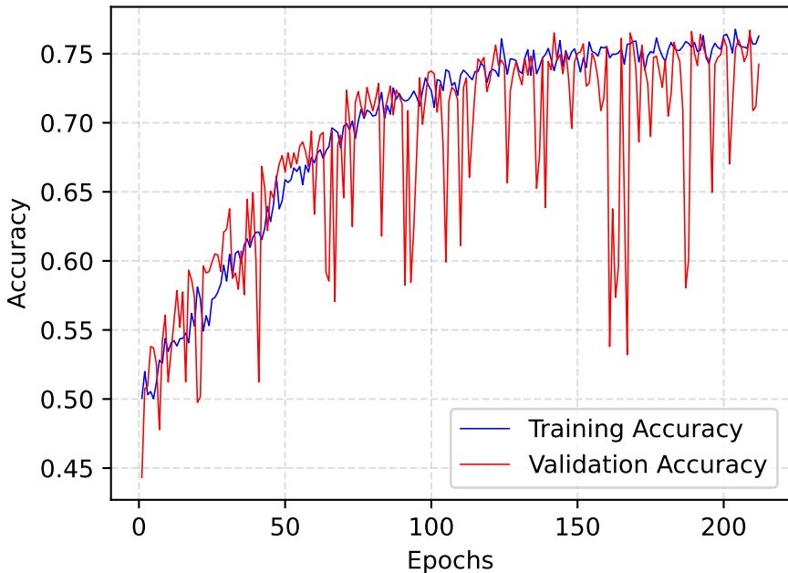
Training VS. Validation Accuracy Quantized-4-Small Model - Tp=9 - Seed=42
