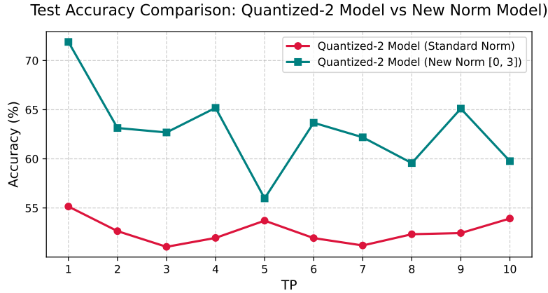
Figure 4.11: Comparative analysis of the 2 -bit quantized basic model under standard normalization vs. advanced Gaussian discrete mapping pipeline.
