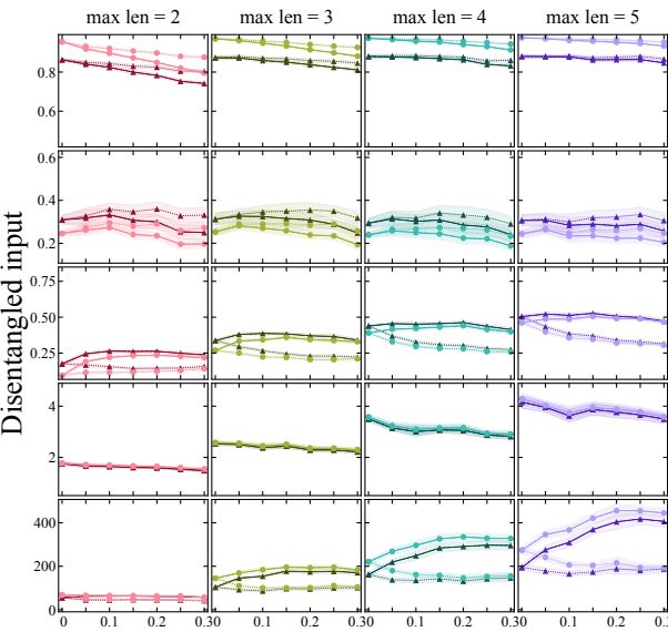
Erasure channel
