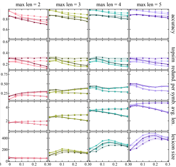
Deletion channel
