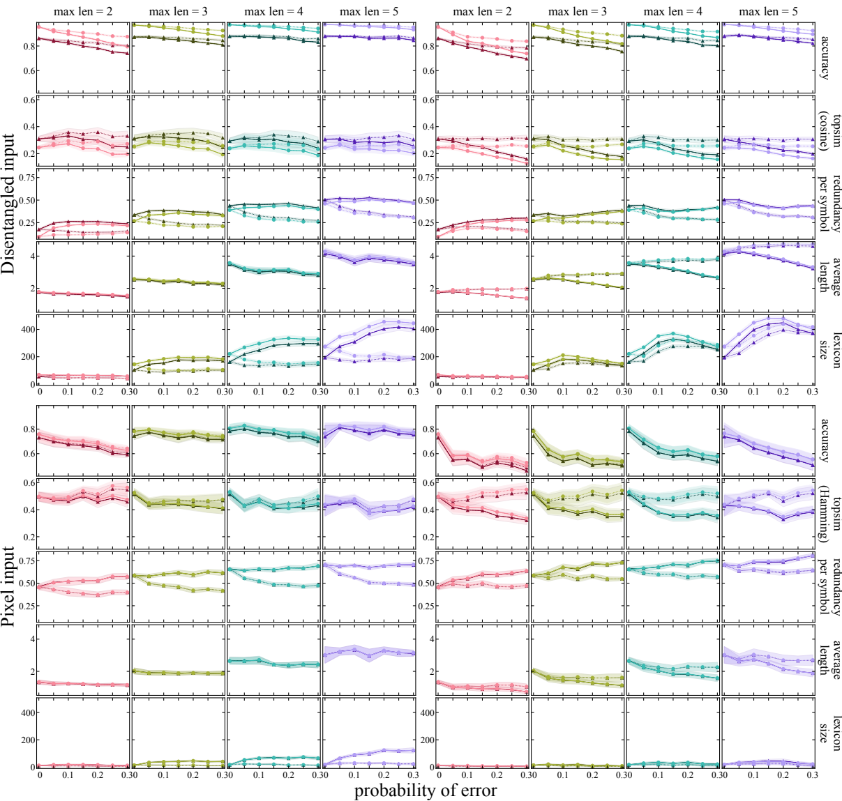
Erasure channel
