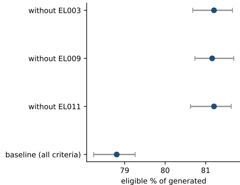
C. Criterion stress test (calibrated, A16)
