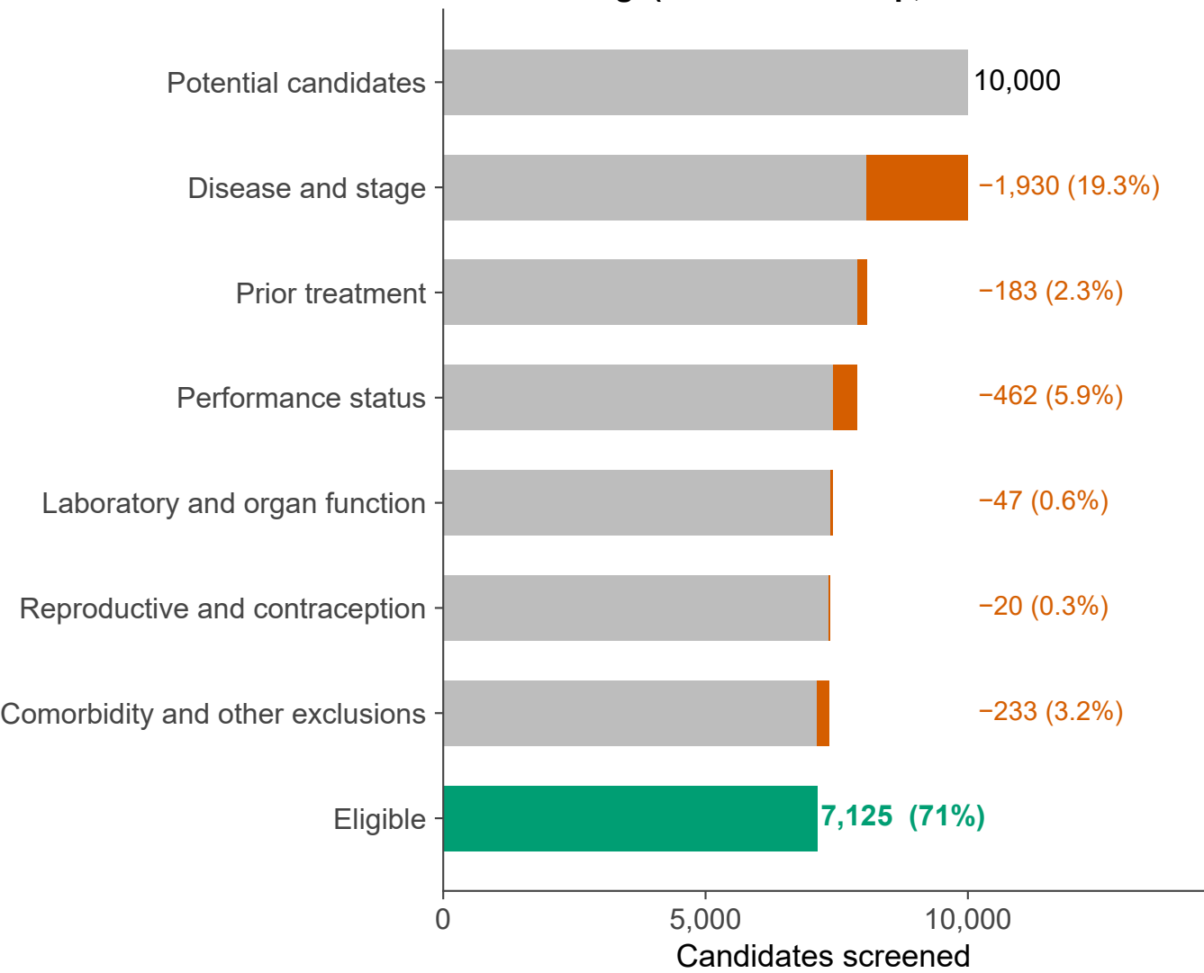
A. Screening (loss at each step, % of those reaching it)
