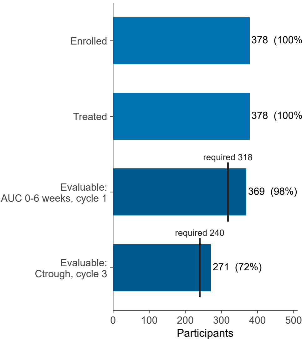
B. After enrolment
