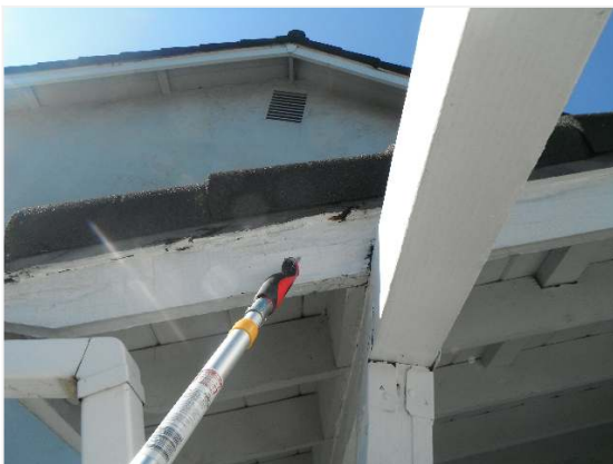
Damaged varge rafter at the front porch.
