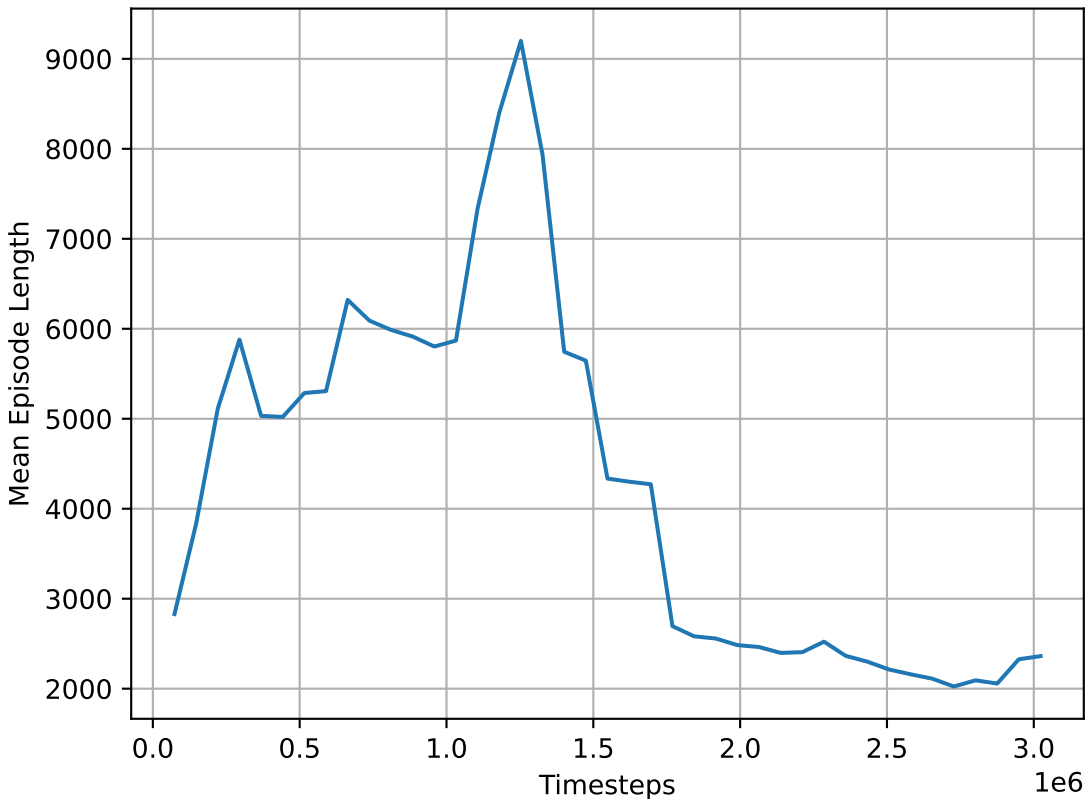
Mean Episode Length Over Time in Training
