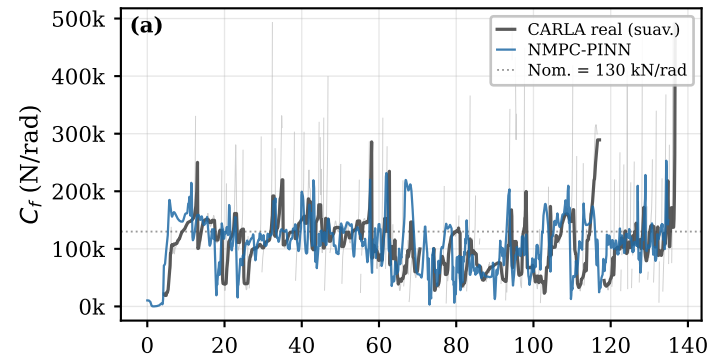
CARLA real vs NMPC-PINN
