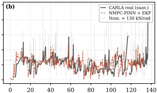
CARLA real vs NMPC-PINN + EKF
