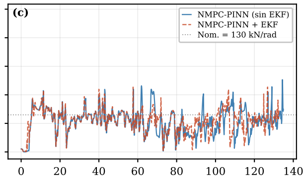
NMPC-PINN vs NMPC-PINN + EKF
