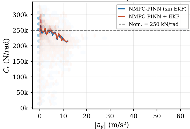
(b) C_r vs |a_y|
