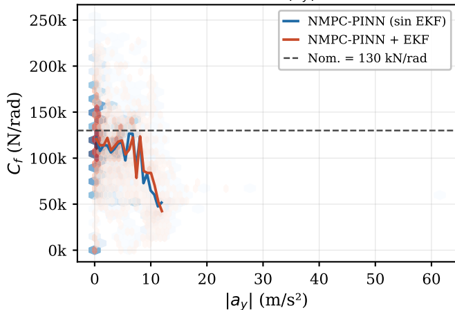
(a) C_f vs |a_y|
