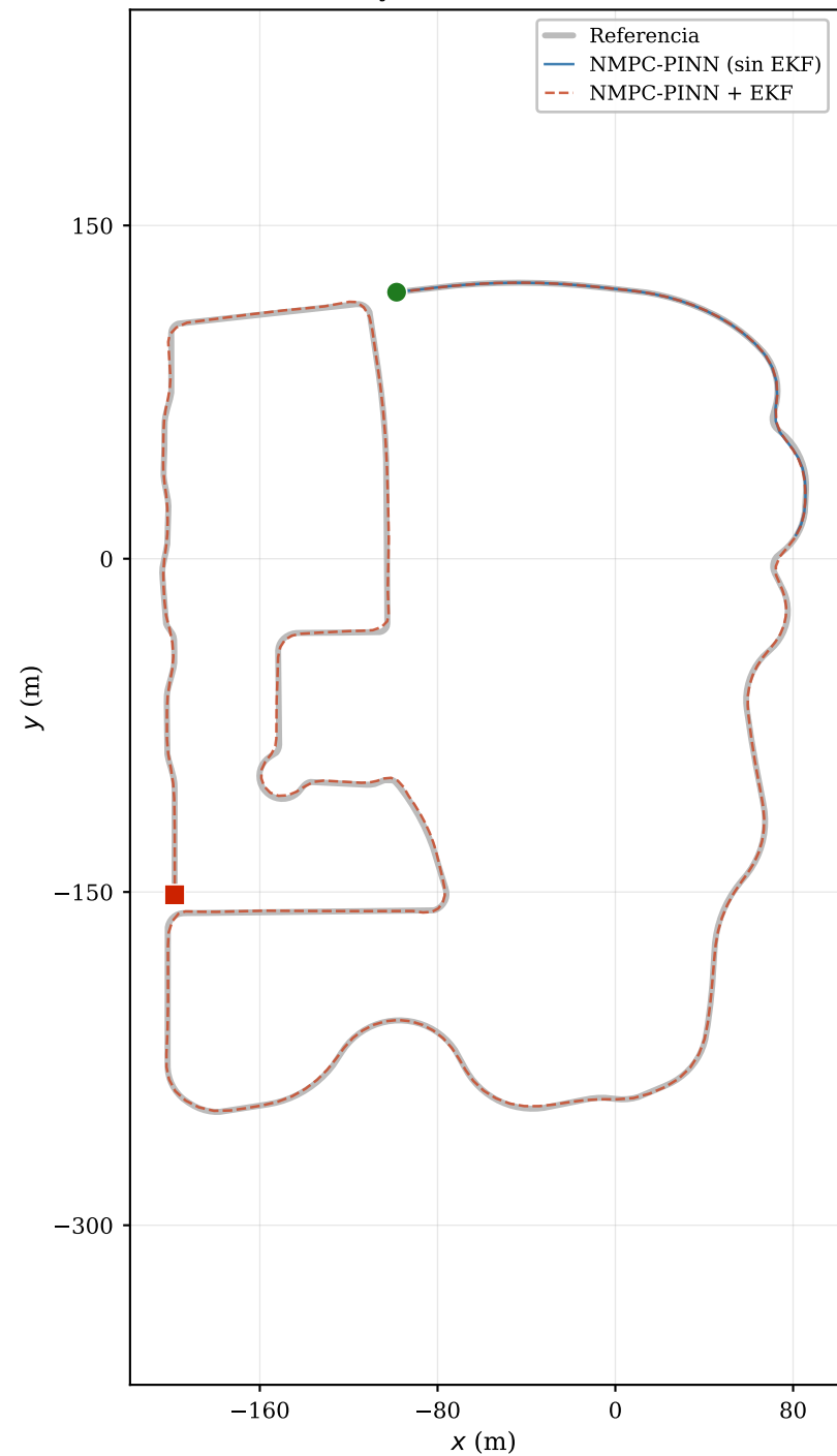
(a) Trayectorias XY — Town07
