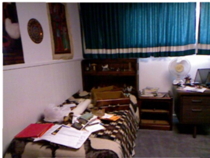
Conv Decoder
