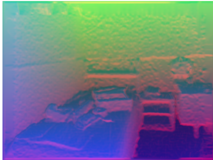
HHA Depth
