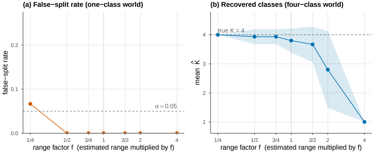
Figure 5: Robustness to a multiplicative error f in the estimated range (area scaling as f^2 ; dotted line marks the unperturbed estimate). (a) The false-split rate on the one-class world stays at zero under any overestimate and reaches only 0.07, near the nominal \alpha , under a four-fold underestimation. (b) Recovery on the four-class world (mean \hat{K} \pm 1 sd) survives underestimation unharmed and degrades only under overestimation, collapsing to silence ( \hat{K} = 1 ), never to invention.
