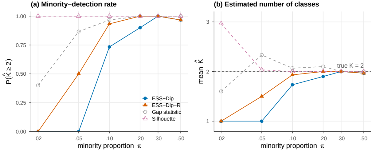
Figure 6: Detection of a contiguous minority class of proportion \pi (true K = 2 ; identical scenes across methods; dashed curves mark the baselines, whose apparent detection is not creditable given their near-one false-split rate on class-free scenes). (a) ESS-Dip detects the minority reliably down to \pi = 0.20 and ESS-Dip-R extends the regime to \pi = 0.10 . (b) At extreme imbalance the silhouette reports \hat{K} \approx 3 by fragmenting the majority class, whereas the calibrated family degrades to silence ( \hat{K} = 1 ).
