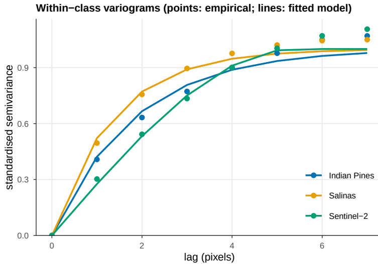
Figure 7: Within-class variograms on the real scenes: the radial empirical semivariogram of the first principal component (points), averaged over pure single-class windows and standardised to unit sill, with the best-fitting exponential, spherical or Gaussian model (lines). The within-class autocorrelation the calibration relies on is real and has a well-defined range on actual imagery.
