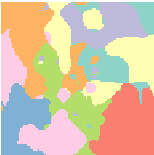
(c) Hennig-Lin ( K = 8 )
