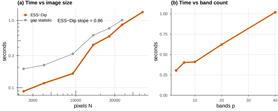
Fig. 3 Computational performance (single-threaded). (a) Wall-clock time versus pixel count N on a log-log scale, with the fitted ESS-Dip scaling exponent; (b) time versus band count p at N = 128^2 .
