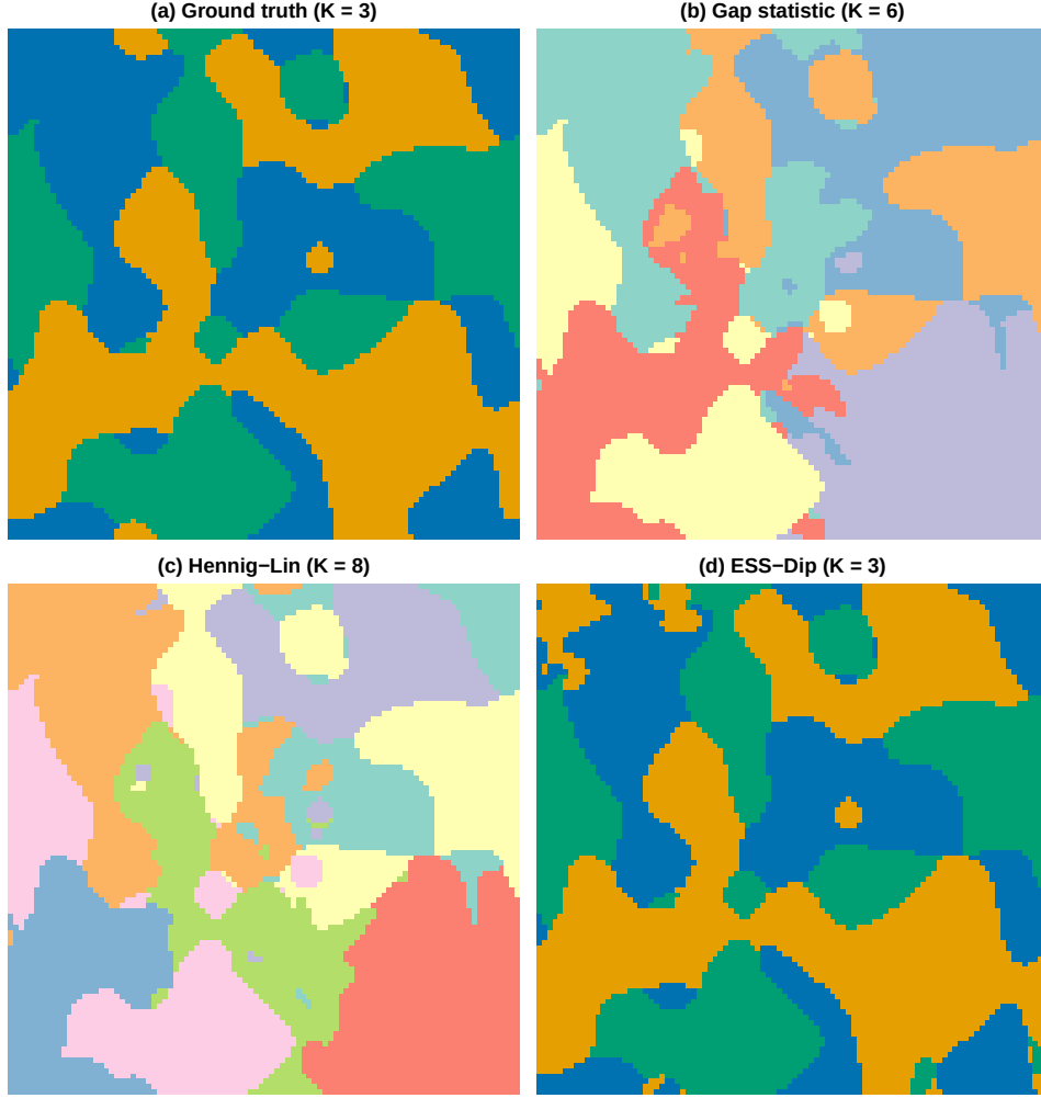
Fig. 2 Recovery on a representative mixed scene (three classes plus a smooth trend). The gap statistic over-segments into six clusters (b) and the Hennig-Lin spatial null into eight (c), both reading the trend and the within-class autocorrelation as extra structure; ESS-Dip removes the trend and calibrates to the effective sample size, recovering the three true classes (d), whose partition matches the ground truth (a). Cluster colours in (b) and (c) are arbitrary; in (a) and (d) they are matched, so a correct recovery reproduces the colours of panel (a).
