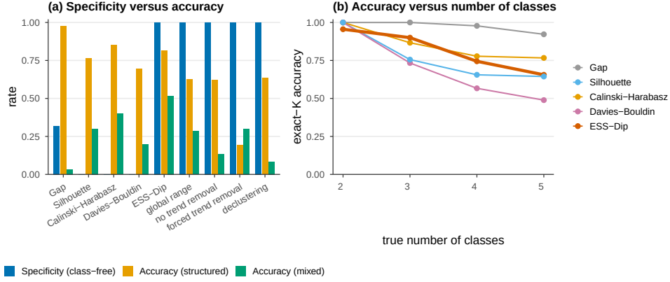
Fig. 1 Left: specificity (class-free scenes) against exact- K accuracy on structured and mixed scenes, by method. Only the proposed family attains unit specificity; among them ESS-Dip recovers the most structure. Right: exact- K accuracy versus the true number of classes on structured scenes. For legibility the panels show the four standard indices and the ESS-Dip family; the calibrated-validity-index and Gaussian-simulation methods of Table 1 are omitted.
