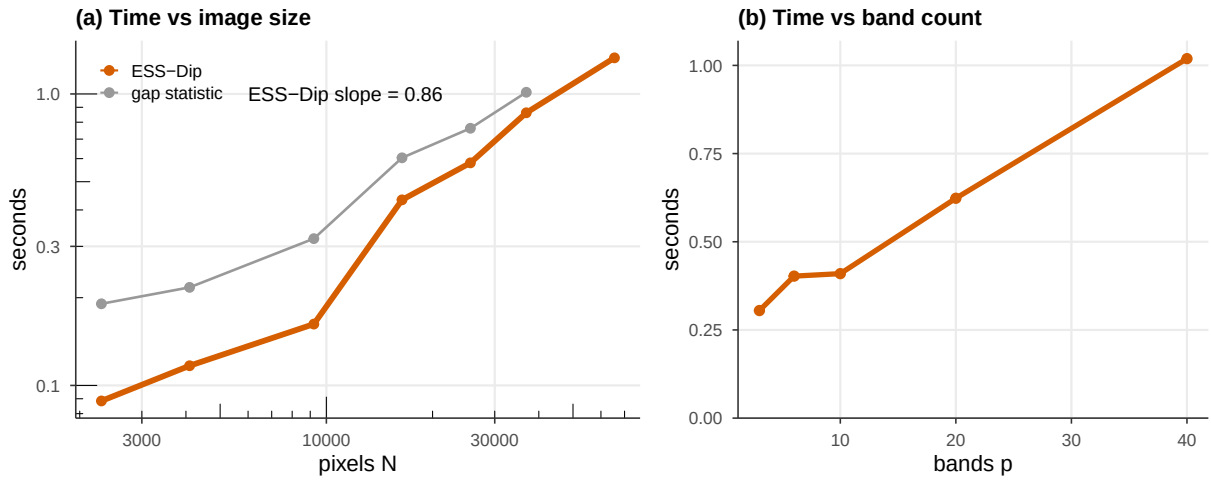
Figure 4: Computational performance (single-threaded). (a) Wall-clock time versus pixel count N on a log-log scale, with the fitted ESS-Dip scaling exponent; (b) time versus band count p at N = 128^2 .
