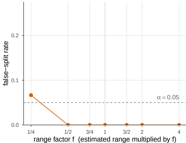
(a) False-split rate (one-class world)
