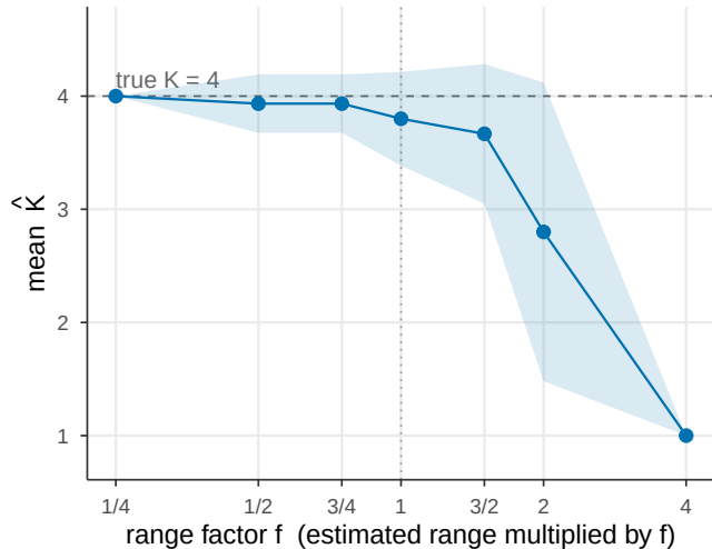
(b) Recovered classes (four-class world)
