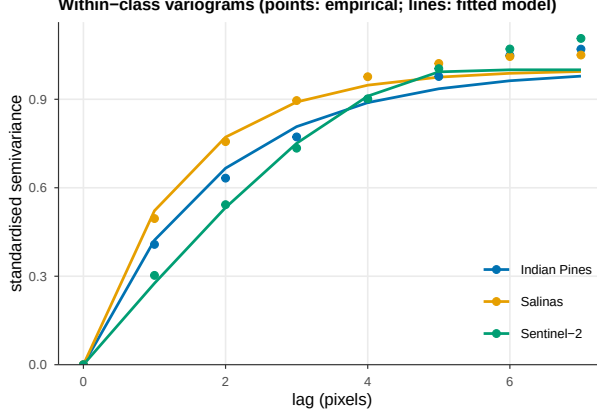
Fig. 7 Within-class variograms on the real scenes: the radial empirical semivariogram of the first principal component (points), averaged over pure single-class windows and standardised to unit sill, with the best-fitting exponential, spherical or Gaussian model (lines). The within-class autocorrelation the calibration relies on is real and has a well-defined range on actual imagery.
