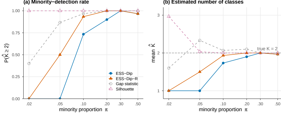
Fig. 6 Detection of a contiguous minority class of proportion \pi (true K = 2 ; identical scenes across methods; dashed curves mark the baselines, whose apparent detection is not creditable given their near-one false-split rate on class-free scenes). (a) ESS-Dip detects the minority reliably down to \pi = 0.20 and ESS-Dip-R extends the regime to \pi = 0.10 . (b) At extreme imbalance the silhouette reports \hat{K} \approx 3 by fragmenting the majority class, whereas the calibrated family degrades to silence ( \hat{K} = 1 ).
