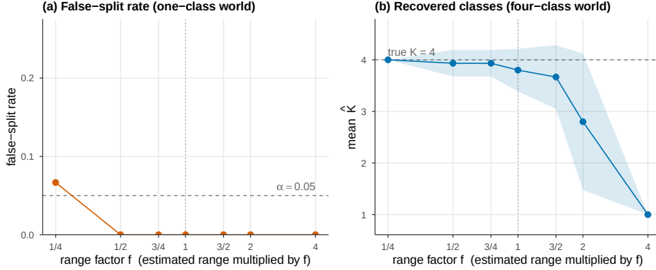
Fig. 5 Robustness to a multiplicative error f in the estimated range (area scaling as f^2 ; dotted line marks the unperturbed estimate). (a) The false-split rate on the one-class world stays at zero under any overestimate and reaches only 0.07, near the nominal \alpha , under a four-fold underestimate. (b) Recovery on the four-class world (mean \hat{K} \pm 1 sd) survives underestimation unharmed and degrades only under overestimation, collapsing to silence ( \hat{K} = 1 ), never to invention.
