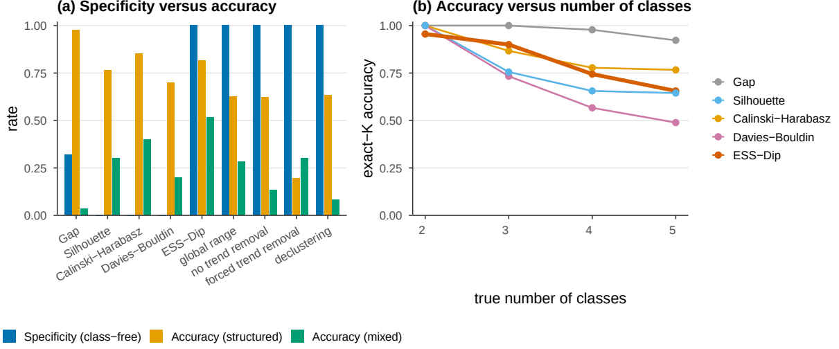
Figure 2: Left: specificity (class-free scenes) against exact- K accuracy on structured and mixed scenes, by method. Only the proposed family attains unit specificity; among them ESS-Dip recovers the most structure. Right: exact- K accuracy versus the true number of classes on structured scenes. For legibility the panels show the four standard indices and the ESS-Dip family; the calibrated-validity-index and Gaussian-simulation methods of Table 1 are omitted.
