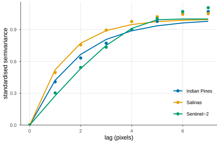
Within-class variograms (points: empirical; lines: fitted model)
