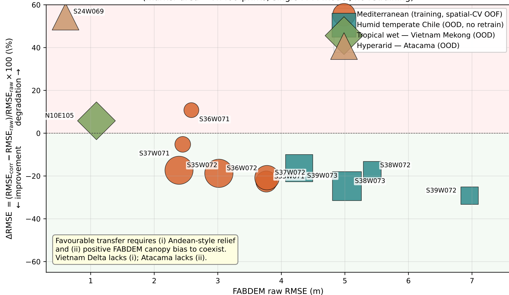
Per-tile correction performance across four climate regimes (marker area \propto \sqrt{n} footprints; single M-M model, no retraining)
