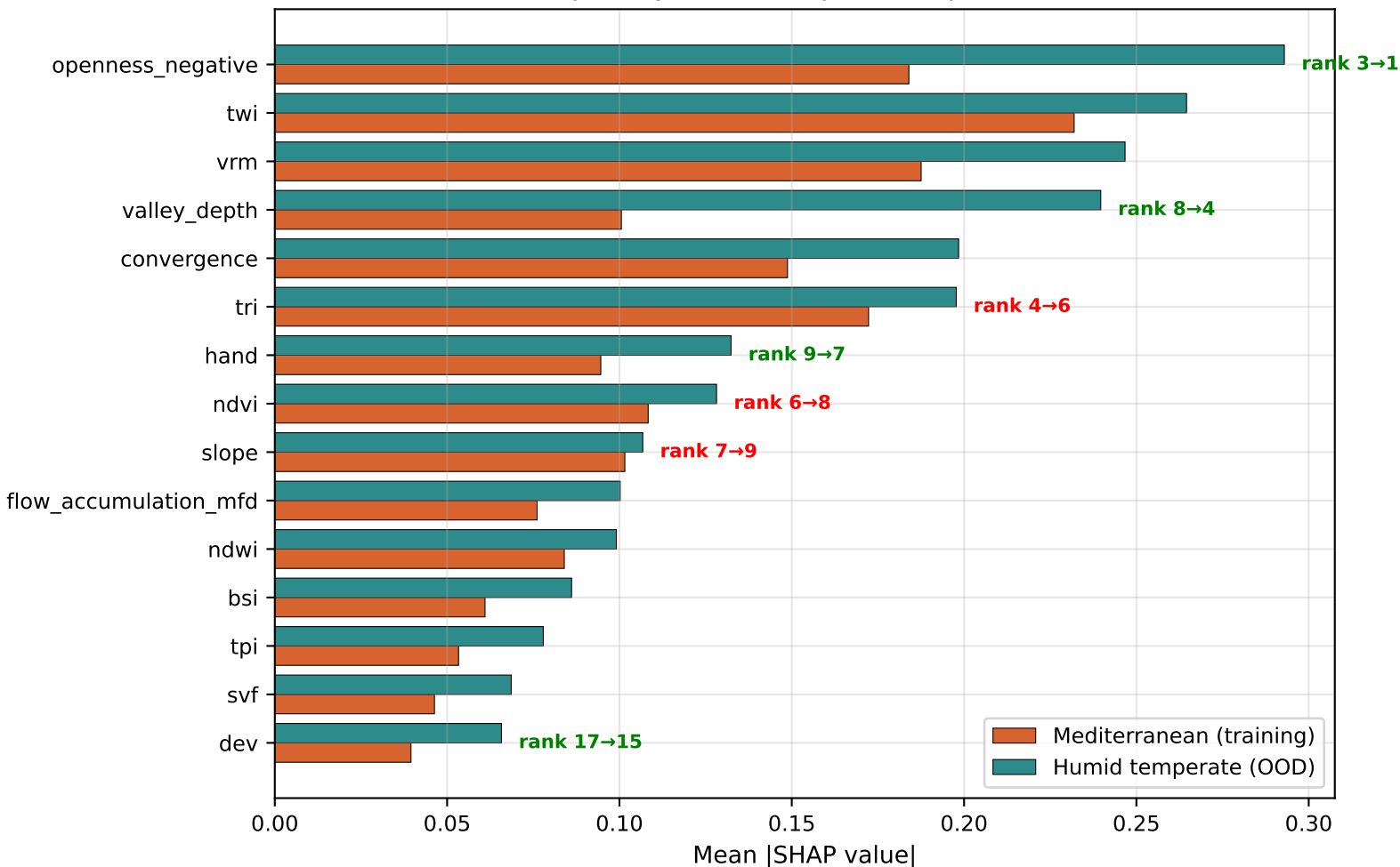
Feature importance shift: same model, two climate regimes (top 15 by humid temperate importance)
