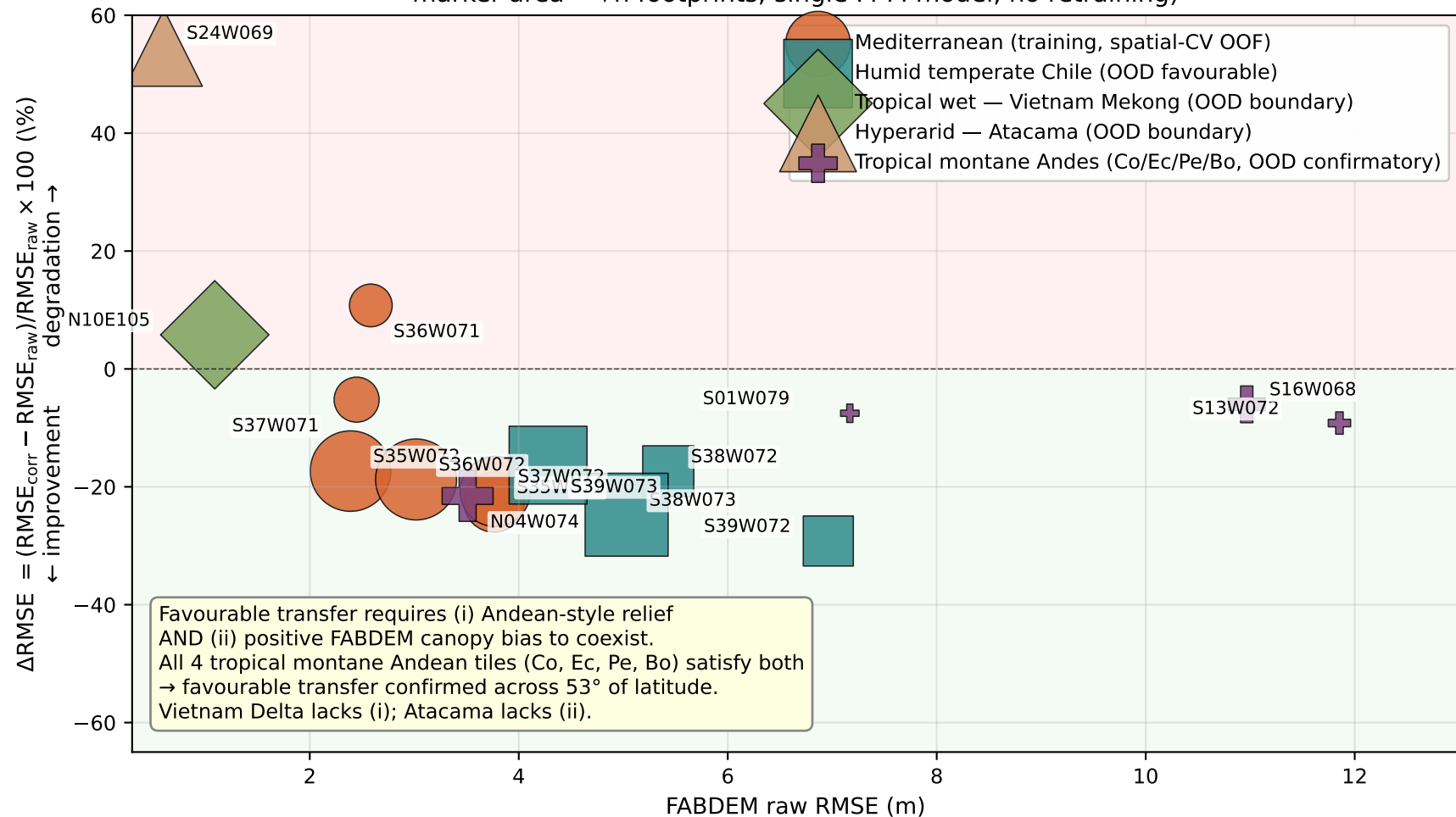
Per-tile correction performance across five climate regimes (tropical montane Andes panel = 4 tiles spanning Colombia 4°N to Bolivia 16°S; marker area \propto \sqrt{n} footprints; single M-M model, no retraining)
