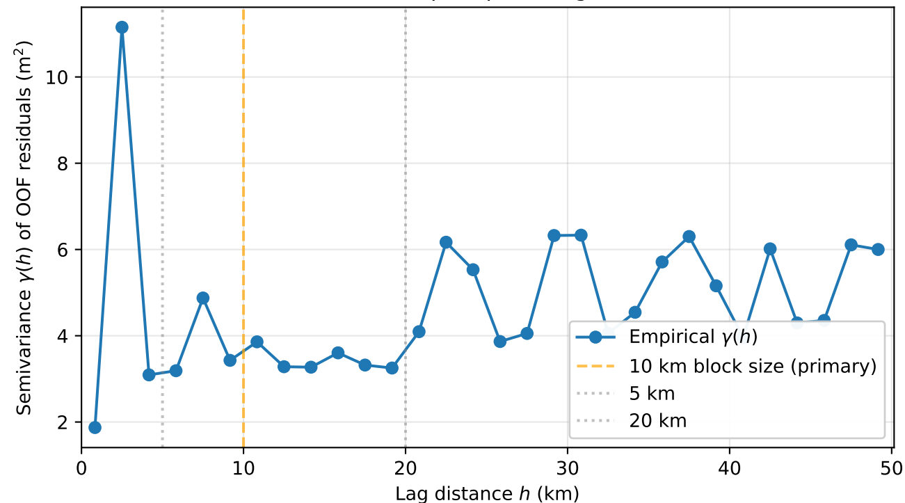
Empirical variogram on Mediterranean OOF residuals (100,356 sampled pairs, lag 0–50 km)
