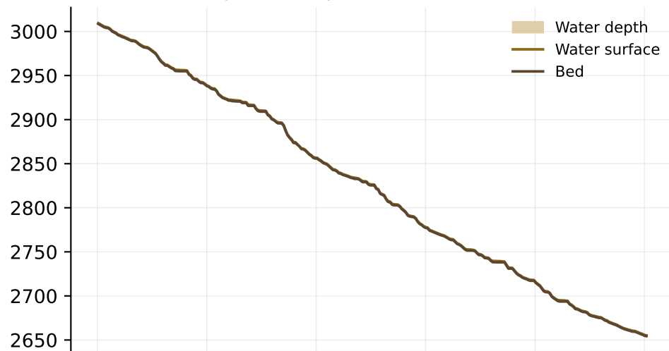
Río Huasco — semiarid Andean (BNA #06) Boulder bed, slope 3.5 %, q = 1 \text{ m}^2/\text{s} , n = 0.06
