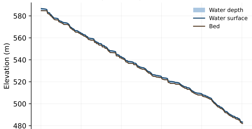
Río Maule — Mediterranean temperate (BNA #11) Andean foothills, slope 1.0 %, q = 3 \text{ m}^2/\text{s} , n = 0.04
