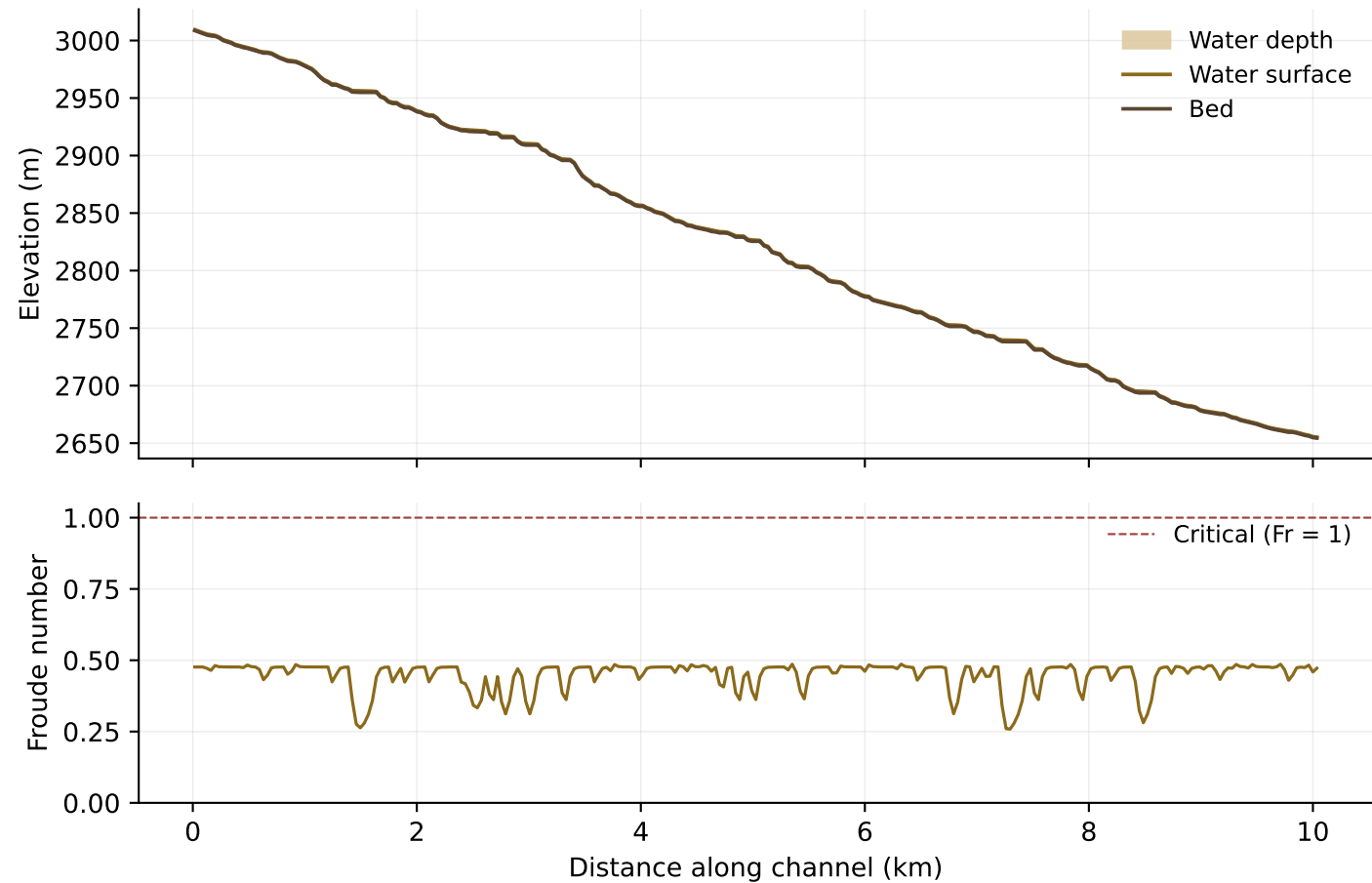
Río Huasco reach — hydroflux-solver-1d steady state ( n = 279 , dx = 36.0 m, q = 1 m 2 /s, n = 0.06 )
